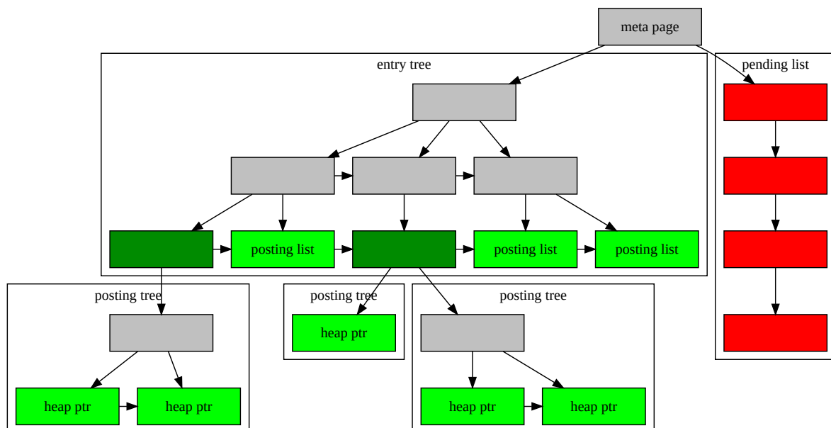
Figure 65.1. GIN Internals
